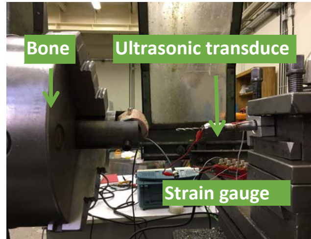
Fig. 1 (a) Overview of testing equipment
