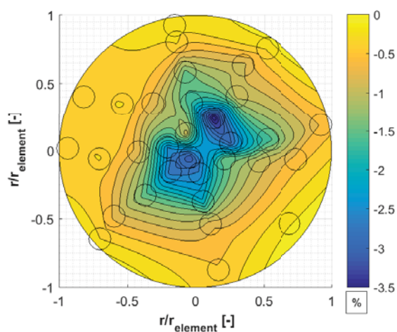
Fig. 12 Isoecho contour for percent change of the surface peak echo amplitude using 1 mm stainless steel ball
