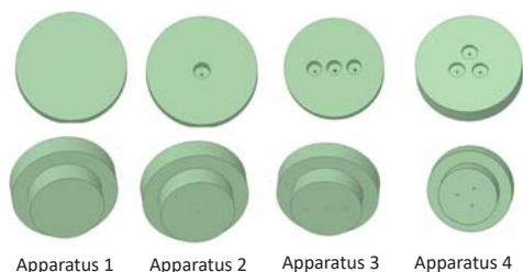
Fig. 15 Bubble injection apparatuses for air injection facility
