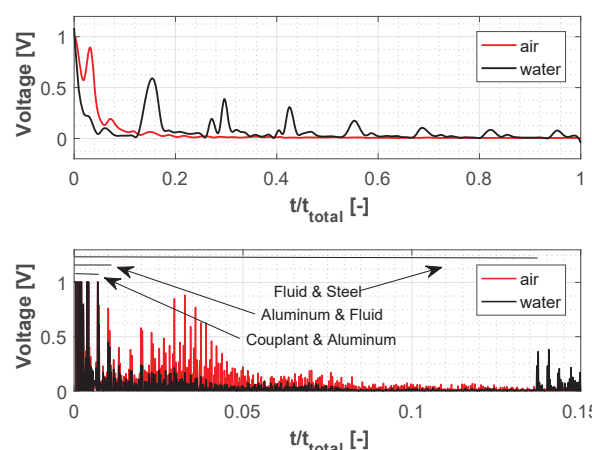
Fig. 13 Front wall reflection characteristics with and without water
