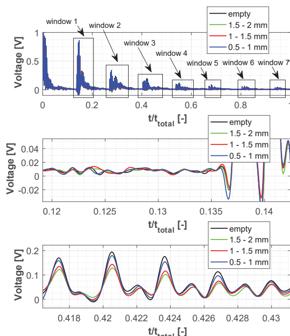
Fig. 16 Single bubble injection experiments applying apparatus 2
