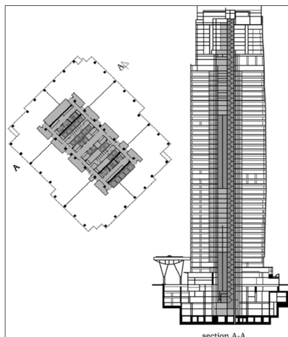
Fig. 15 Midtown Tower: floor plan and section
