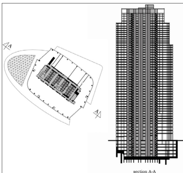
Fig. 13 Toranomom Hills Residential Tower: floor plan and section
