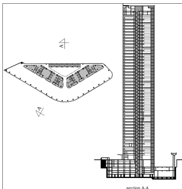
Fig. 3 Dentsu Tower: floor plan and section
