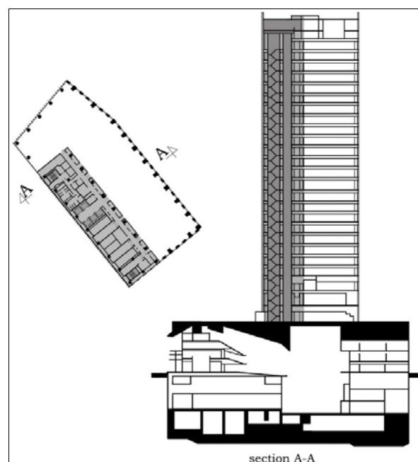
Fig. 5 Ginza Kabukiza: floor plan and section
