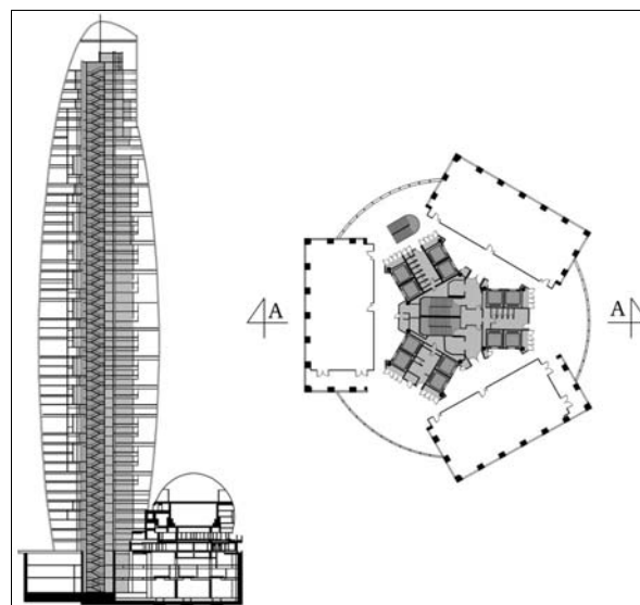
Fig. 7 Mode Gakuen Cocoon Tower: plan and section
