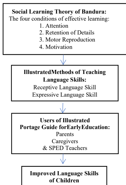
Fig. 1 Theoretical/Conceptual Framework
