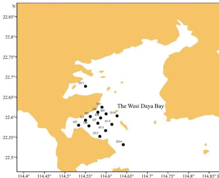
Fig. 1 Survey distribution in the West Daya Bay
