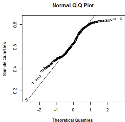
Fig. 2 Quantile-quantile plots of GLM
