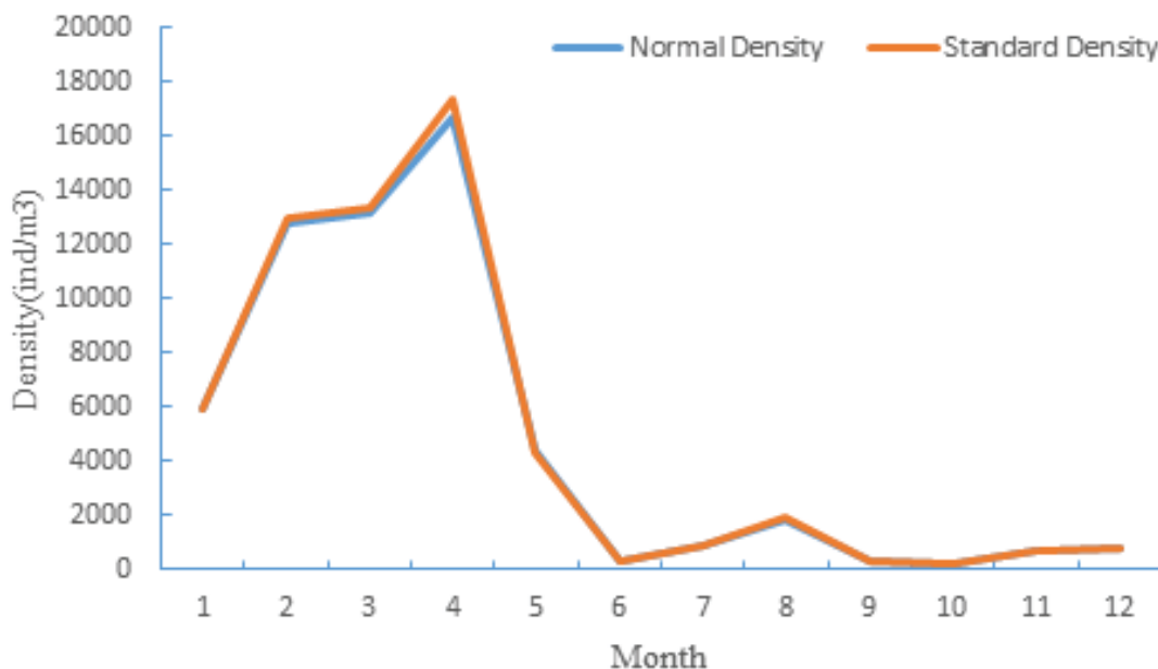
Fig. 8 Comparing standardized density and nominal density of zooplankton in different month
