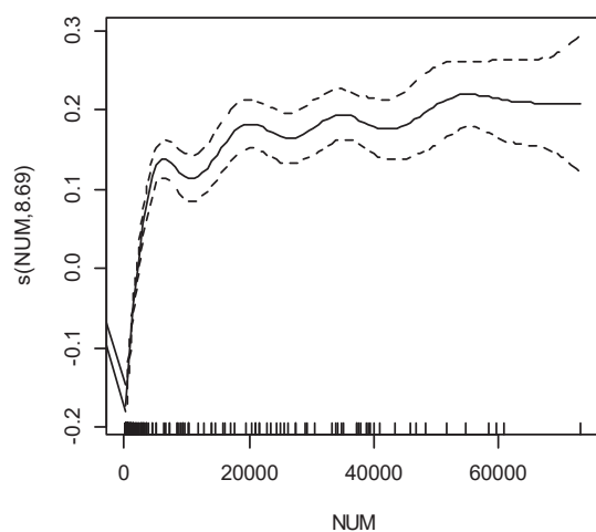
Fig. 6 Effects of the total number of zooplankton capture on the density of zooplankton in the West Daya Bay
