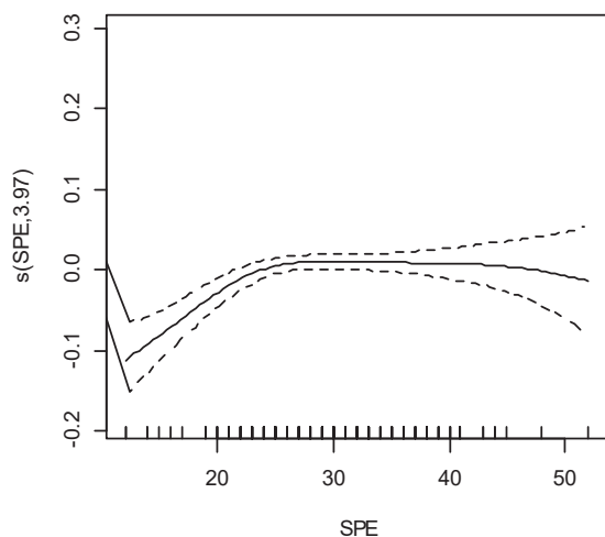
Fig. 5 Effects of the number of zooplankton species captured on the density of zooplankton in the West Daya Bay
