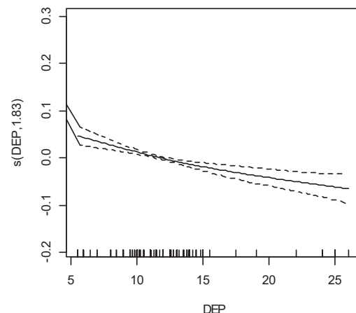
Fig. 4 Effects of the depth of water column on the density of zooplankton in the West Daya Bay
