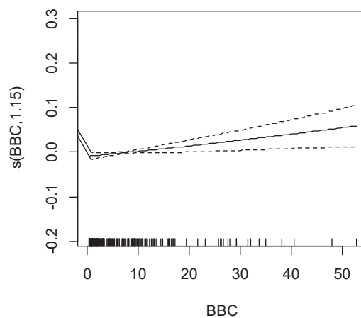
Fig. 3 Effects of the benthonic concentration of chlorophyll a on the density of zooplankton in the West Daya Bay
