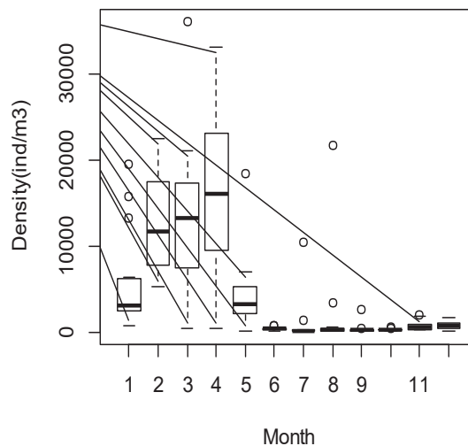
Fig. 7 Effects of the survey month on the density of zooplankton in the West Daya Bay
