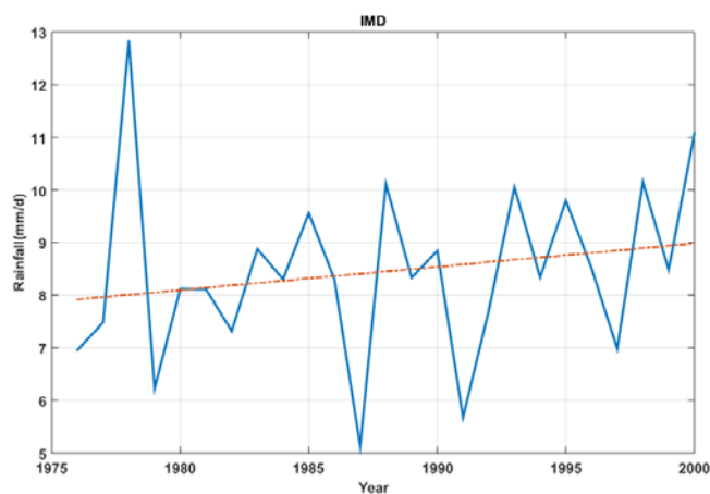
Fig. 5 TS plot for IMD gridded rainfall data over UK for the historical period (1976-2000)
