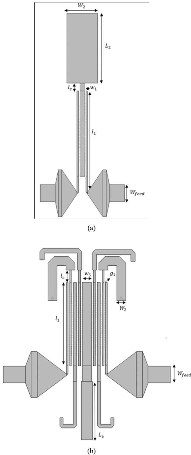
Fig. 2 Geometry of (a) second-order, (b) eighth-order filter
