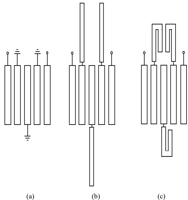
Fig. 1 (a) Conventional interdigital filter, (b) Stage one of the modifications with quarter wavelength open circuit stub, and (c) the modified filter with a compact size
