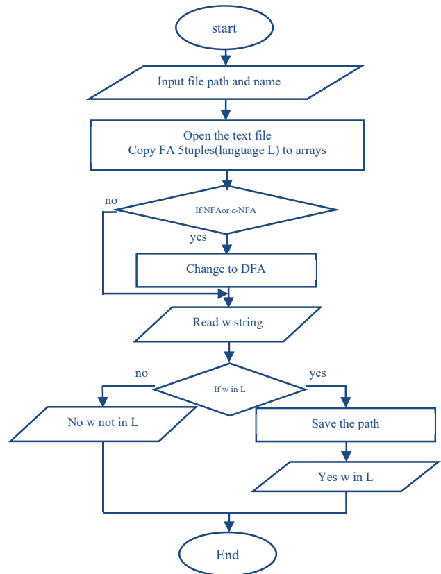
Fig. 10 Program flowchart
