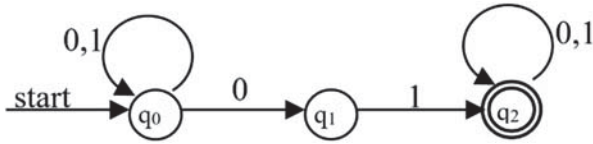
Fig. 2 An NFA for L(A) = \{x01y : x,y \text{ in } \{0,1\}^*\}
