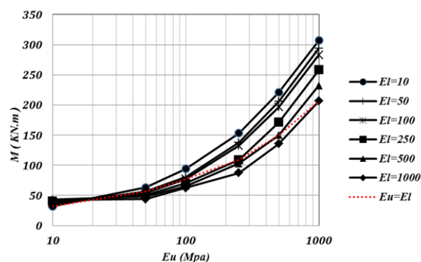
Fig. 4 Bending moment of the tunnel structure in case the interface of the two layers is located at tunnel crest level
