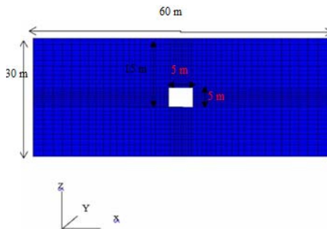
Fig. 2 Model geometry
