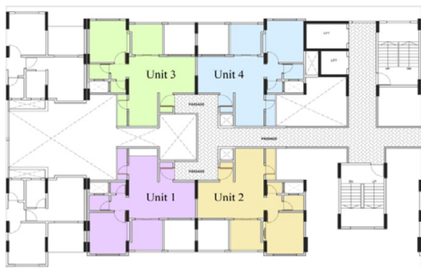
Fig. 3 Schematic Plan of four units
