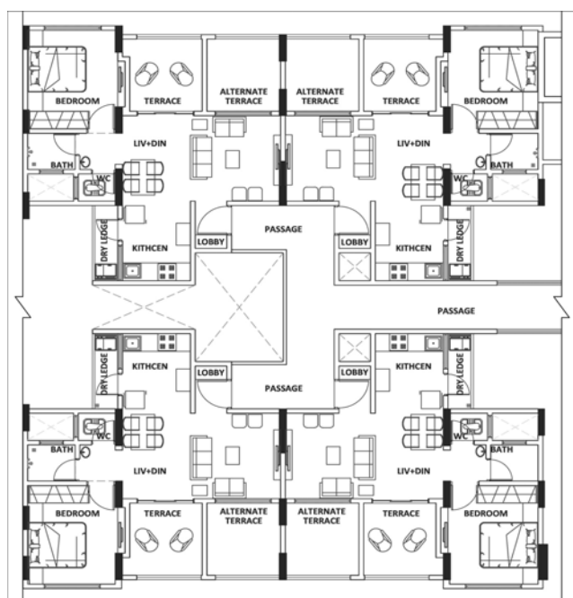
Fig. 4 Even Floor Plan
