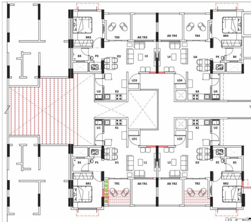
Fig. 12 Design solution proposed for 45-degree
