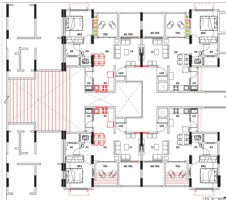
Fig. 13 Design solution proposed for 315-degree WIA
