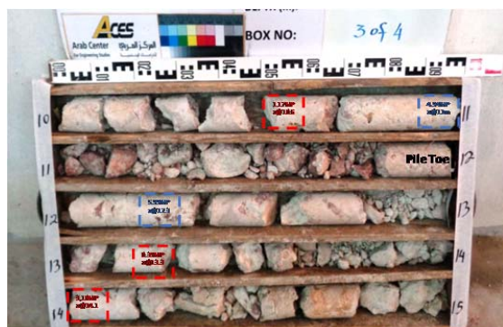
Fig. 5 Core Photo between 10 and 15m depth
