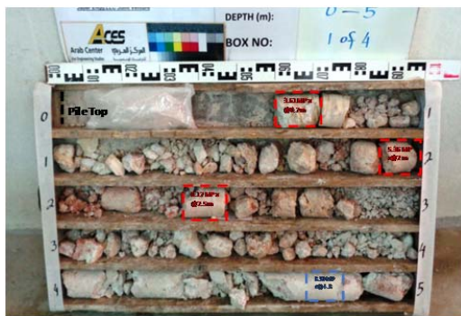
Fig. 2 Core photo between 0 and 5m depth
