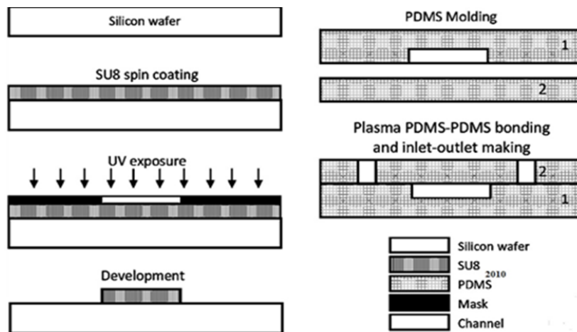
Fig. 3 Fabrication steps for PDMS micro mixer [26]
