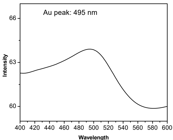
Fig. 10 UV visible spectroscopy result
