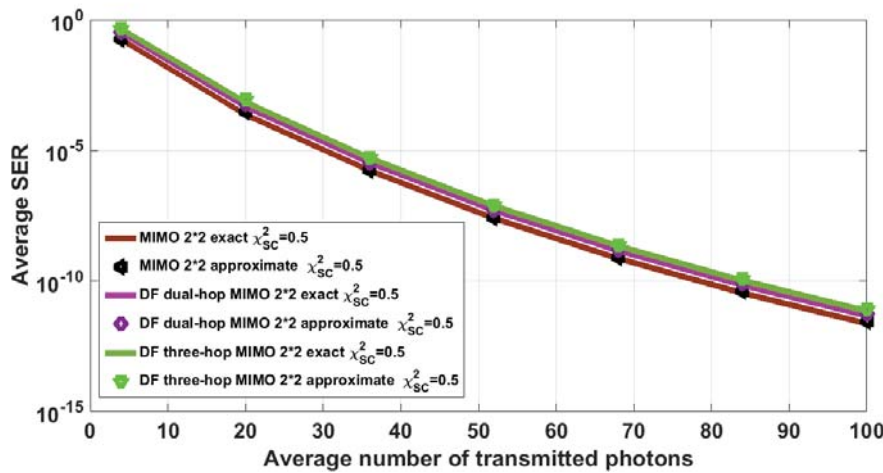
Fig. 3 Comparison between N hops DF relaying MIMO-FSO system under moderate turbulence
