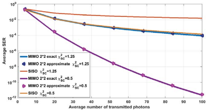
Fig. 2 Comparison of MIMO schemes FSO link by changing the number of transmitters and receivers under strong and moderate turbulence
