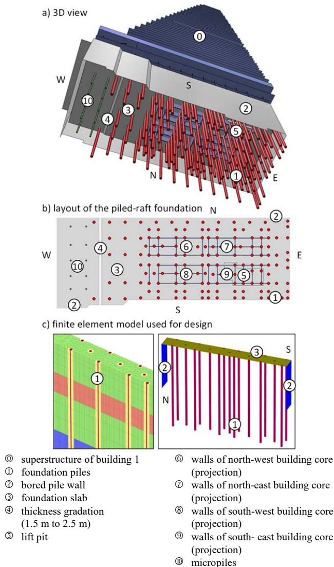
Fig. 5 Foundation layout and numerical modelling
