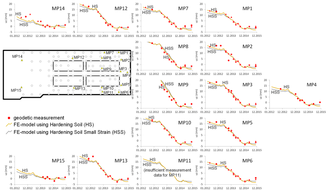
Fig. 7 Measurements and modelled behaviour (settlements vs time)
