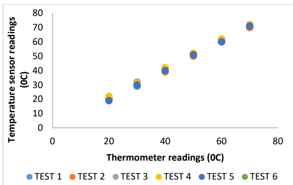
Fig. 4 Calibration of temperature sensor
