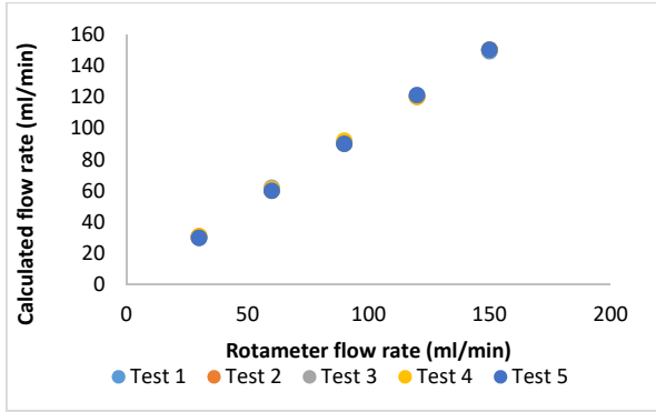
Fig. 3 Calibration of rotameter
