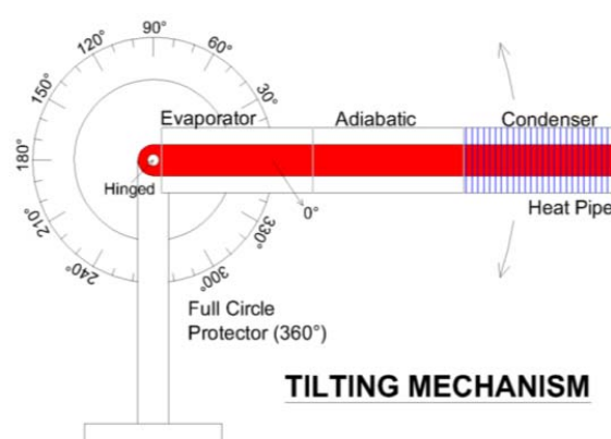
Fig. 2 Schematic diagram of tilting mechanism
