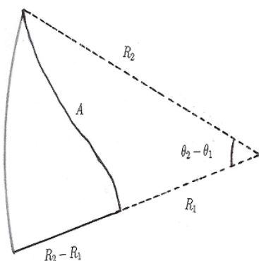
Fig. 1 A curve A with finite length
