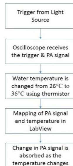
Fig. 2 Workflow of temperature controlled PA system
