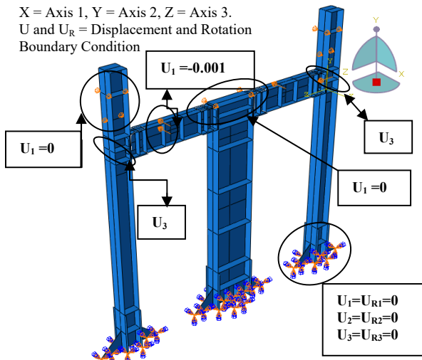
Fig. 4 Boundary conditions
