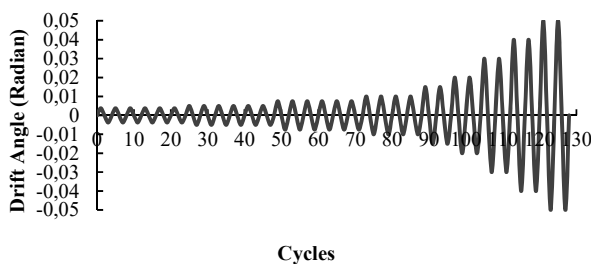
Fig. 2 Cyclic load protocol [8]
