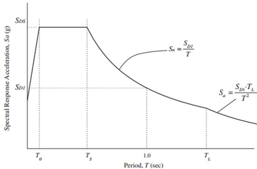
Fig. 2 The acceleration response spectrum [7]
