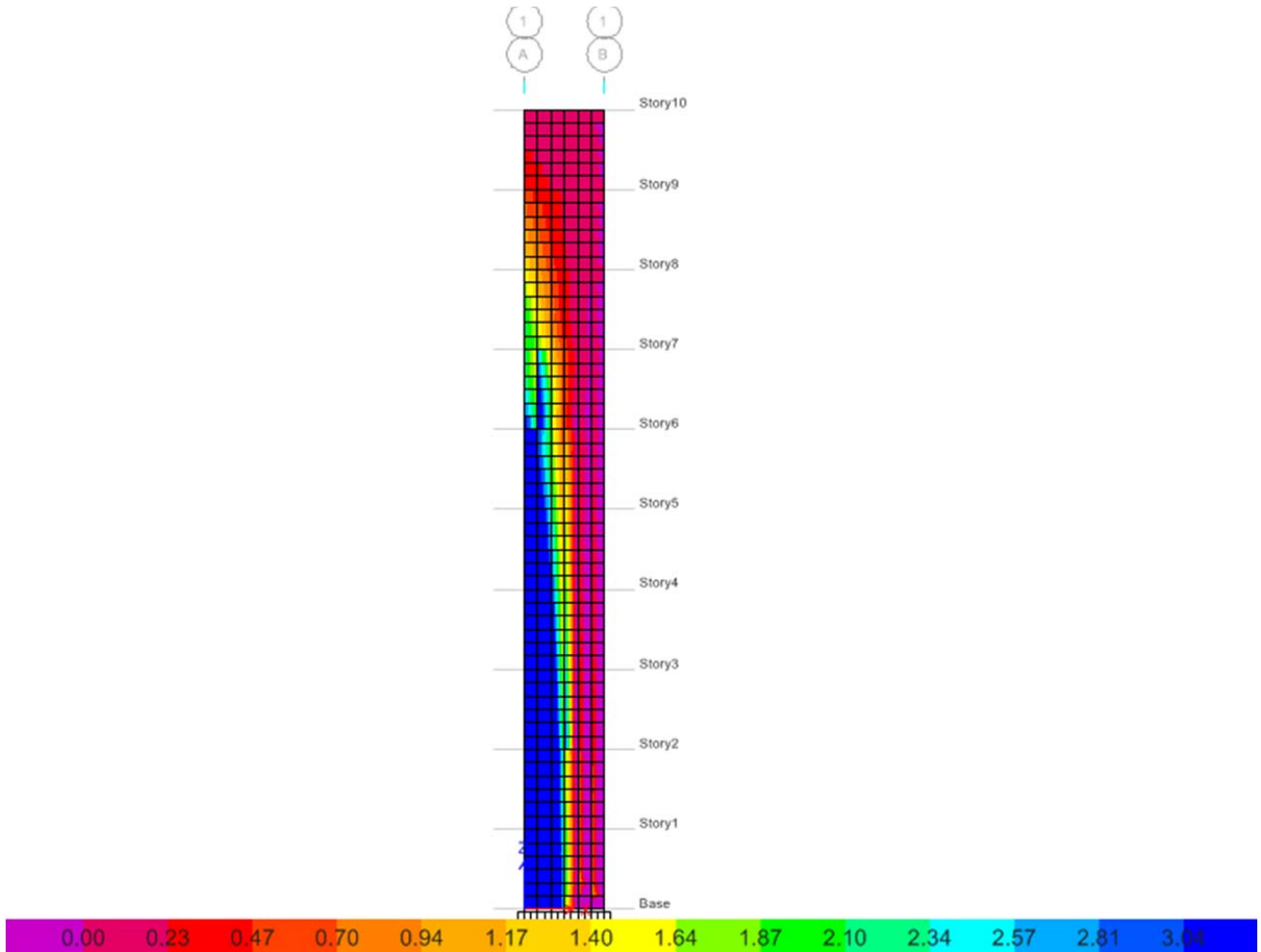
Fig. 6 The maximum tensile stresses in elements due to lateral load for the third step analysis in MPa
