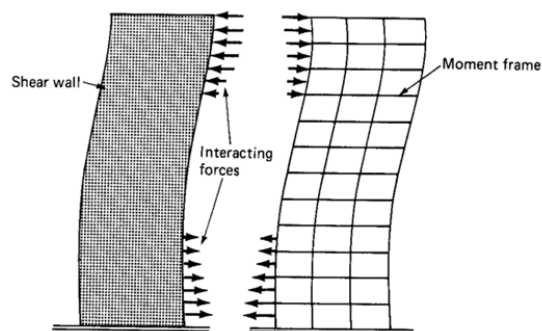
Fig. 1 Shear Wall-Frame interaction [6]
