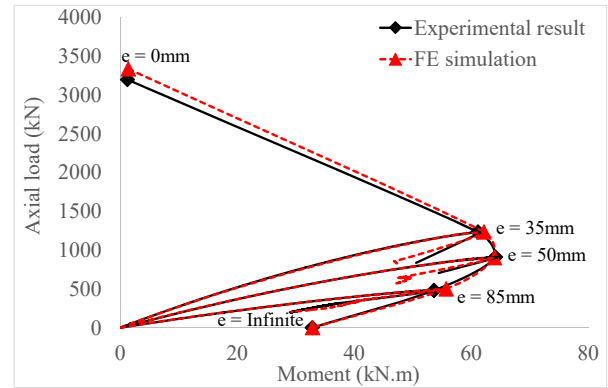
Fig. 10 Load-Moment interaction diagram for UHPFRC slender columns
