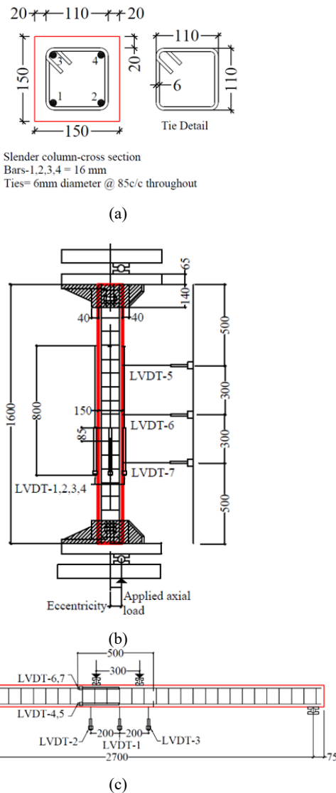
Fig. 2 Test specimen details and instrumentation set up: (a) cross-section of the beam and columns; (b) concentrically and
