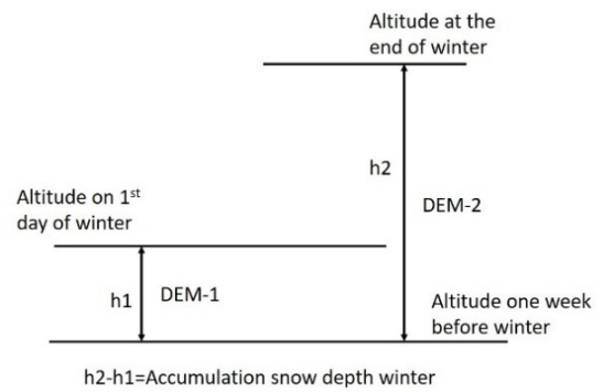
Fig. 2 Illustration of snow depth estimation
