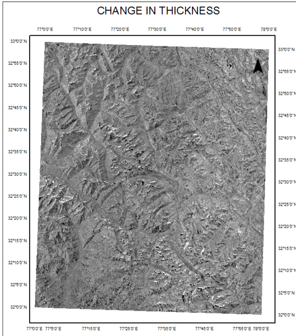
Fig. 5 Change in thickness for 11 years (2000-2011)
