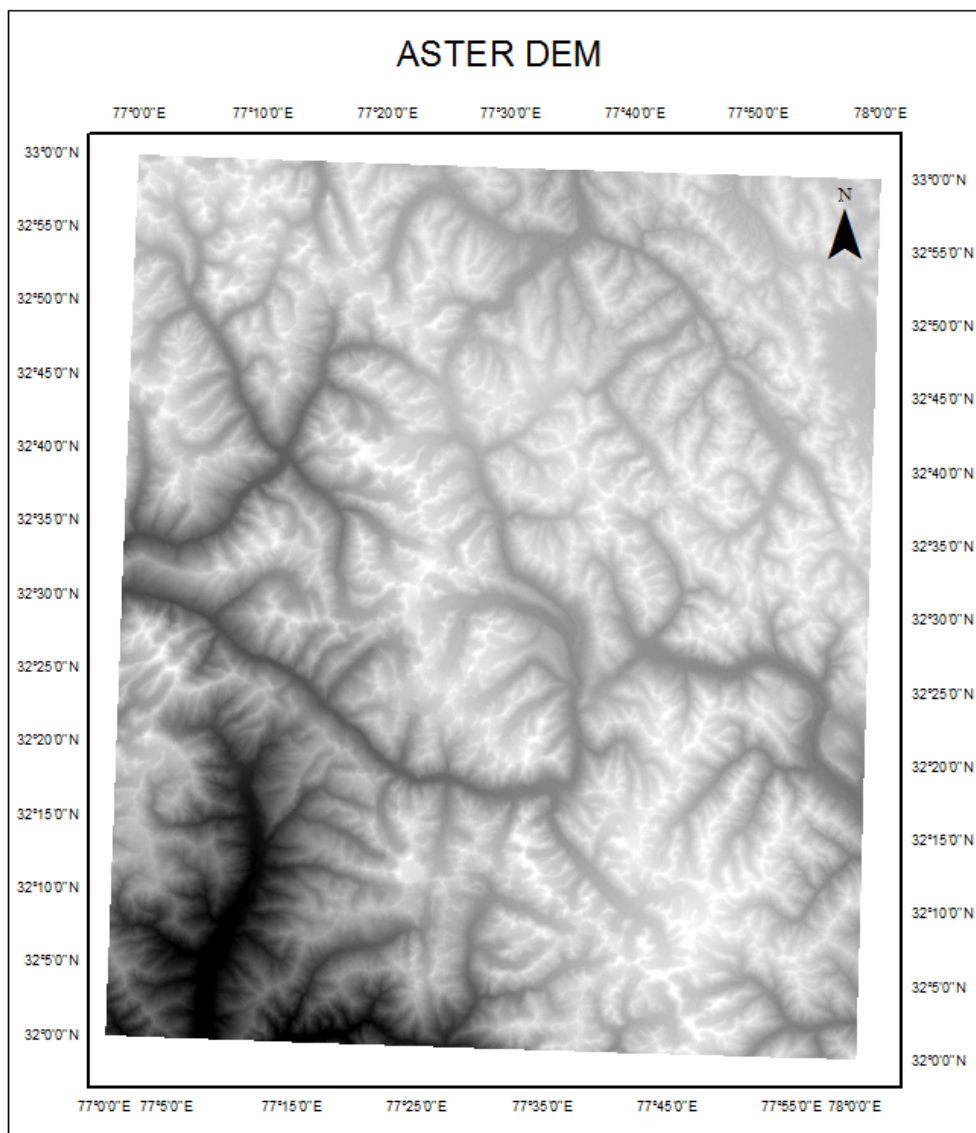
Fig. 4 ASTER DEM - October 2011
