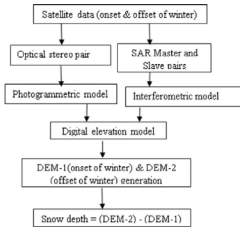
Fig. 1 Methodology suggested for estimating snow depth
