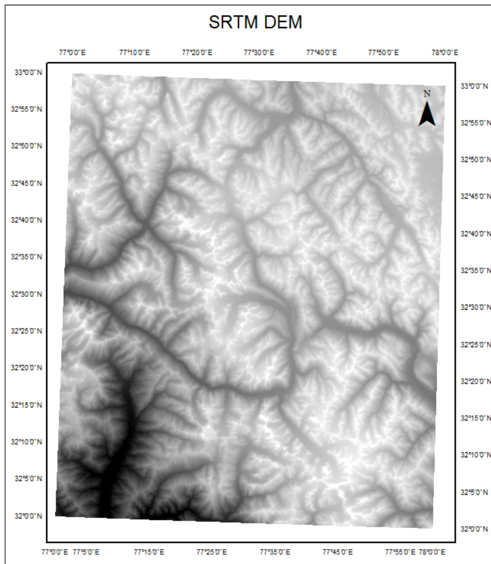
Fig. 3 SRTM DEM - February 2000
