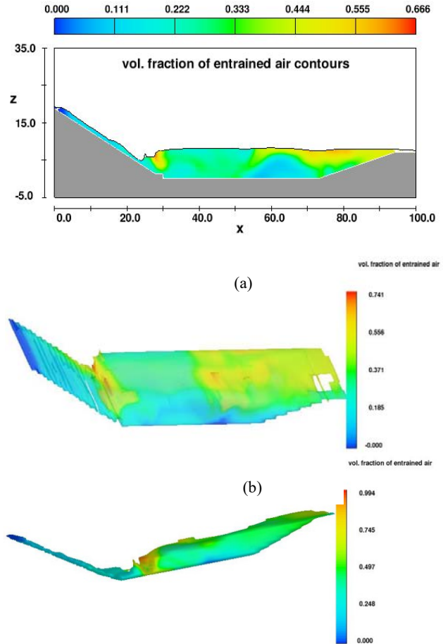
Fig. 11 Simulation of Fraction of entrained air in USBR II stilling basin with end adverse slope– (a) RNG Model, (b) k-ε Model
