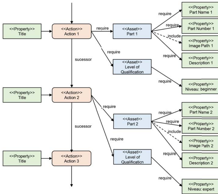
Fig. 3 Inclusion of part variety and qualification levels with the ADAPT-approach
