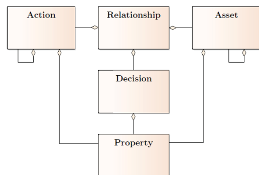
Fig. 2 Five elements of the ADAPT-modelling approach [15]
