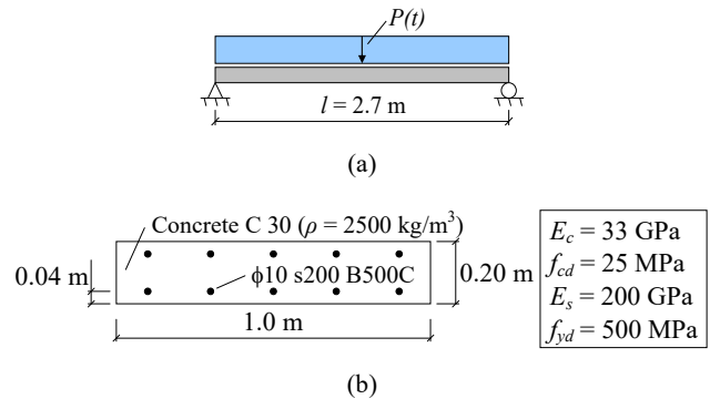
Fig. 6 Studied wall strip subjected to explosion load, (a) showing boundary conditions and (b) showing the cross-section
