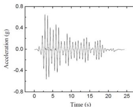
Fig. 3 Input earthquake
