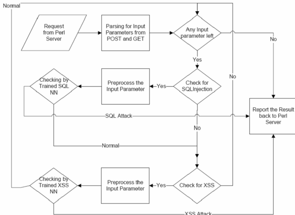
Fig. 4 General Processing Flowchart of ANNbWAF
