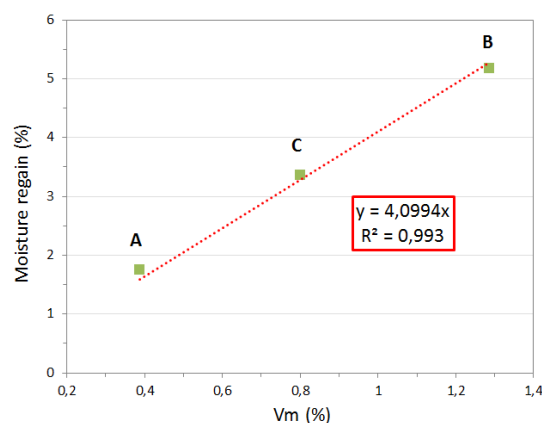
Fig. 7 Linear correlation between V_m and moisture regain
