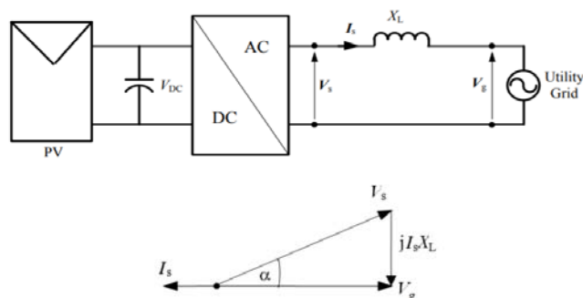
Fig. 2 Inverter equivalent circuit connected to utility grid and phasor diagram [9]
