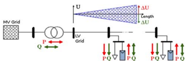
Fig. 1 Illustration of Voltage fluctuation in LV system [6]
