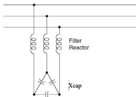
Fig. 16 Filter configuration [10]
