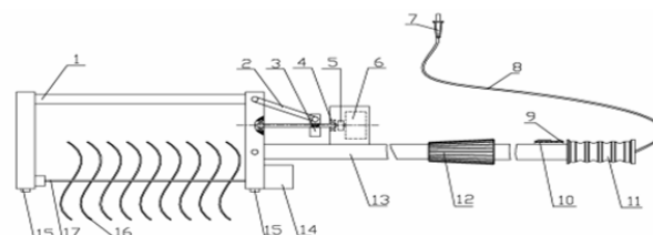
Fig. 10 CN102217493 (A): “Ultrasonic targeted electric flower and fruit thinning machine” [27]
