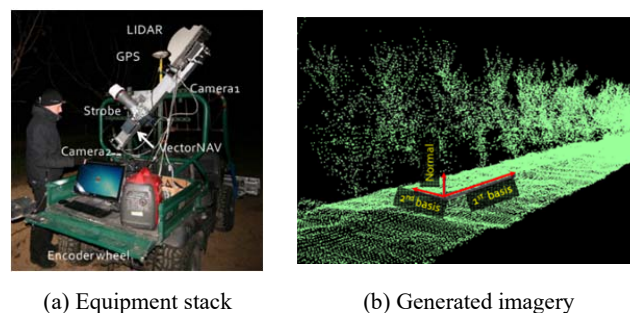
(a) Equipment stack (b) Generated imagery Fig. 16 LIDAR system for orchard mapping, sensor and feature extraction [54]
