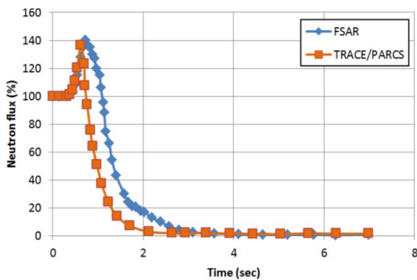
Fig. 3 The neutron flux results
