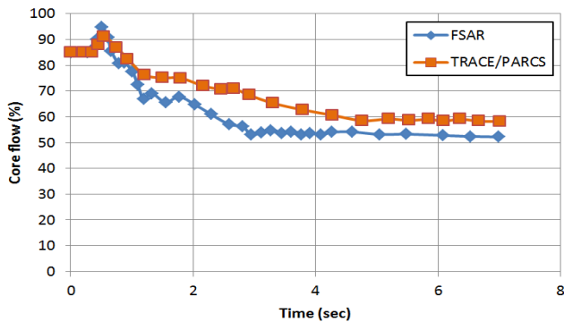
Fig. 6 The core flow results
