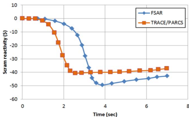
Fig. 4 The scram reactivity results
