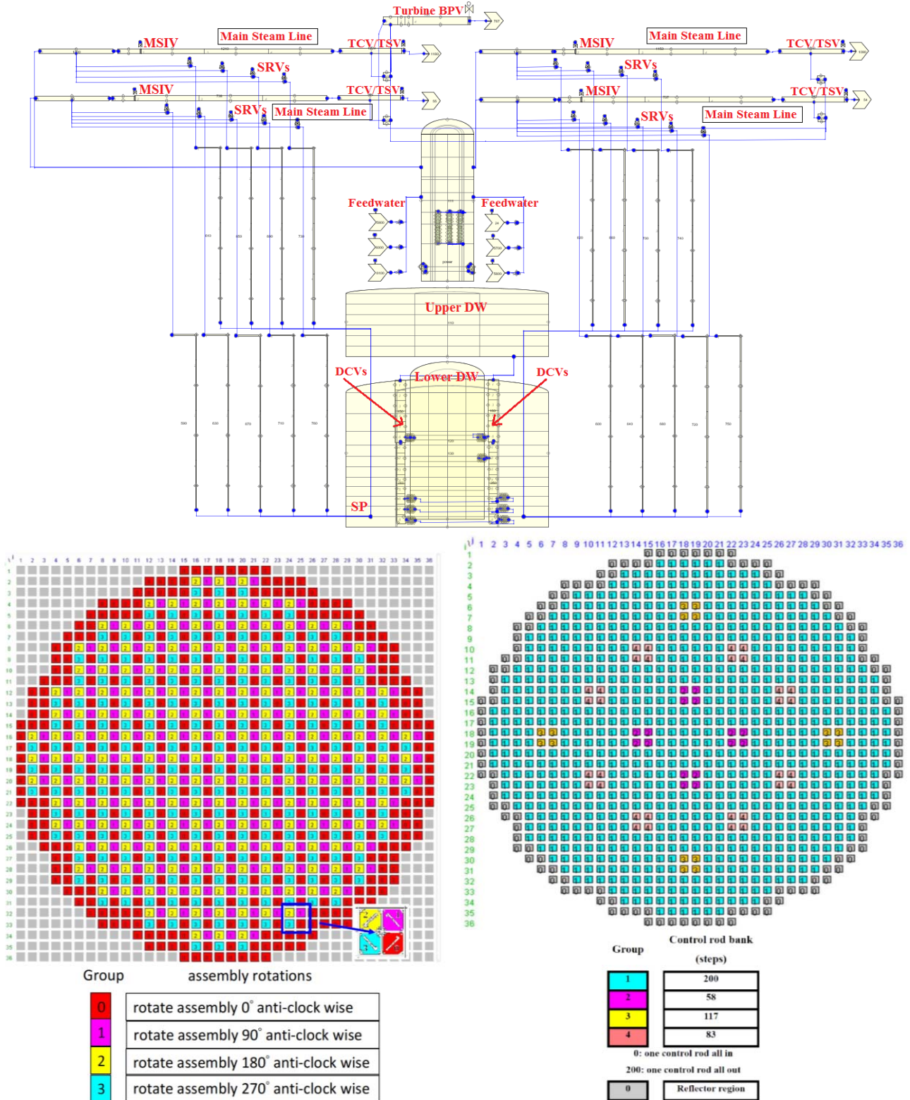
Fig. 2 The TRACE/PARCS/SNAP model of ABWR
