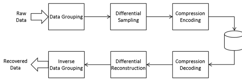
Fig. 4 Compression block diagram of the proposed data recording for in-vehicle network
