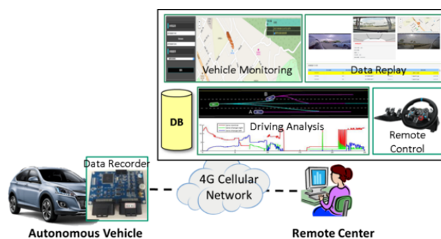
Fig. 1 Remote monitoring of autonomous vehicles
