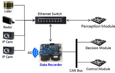
Fig. 2 Heterogeneous architecture of in-vehicle network
