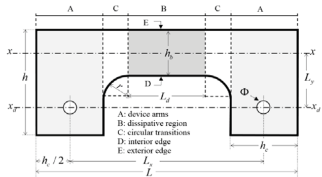
Fig. 1 C-device proposed by [6]
