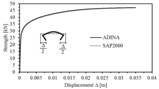
Fig. 15 Comparison of a FE analysis predictions
