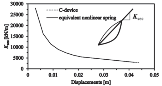
Fig. 7 Comparison of predicted stiffness degradation using different device models under reversed cyclic loading
