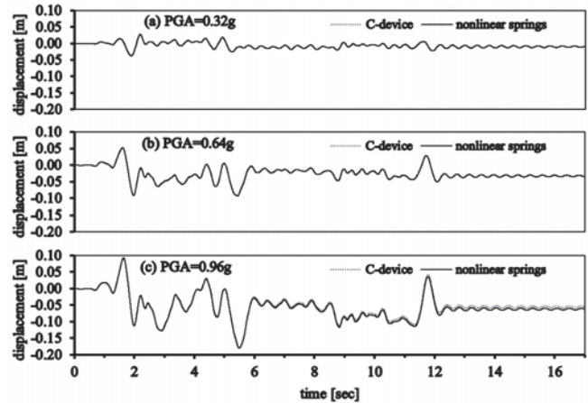
Fig. 12 Comparison of displacement response time-history of the cantilever column with C-devices for two different device models under El Centro EGM scaled at three intensity levels
