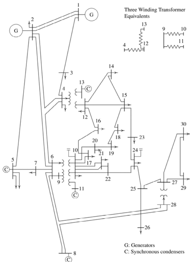
Fig. 1 IEEE 30 Bus Test System
