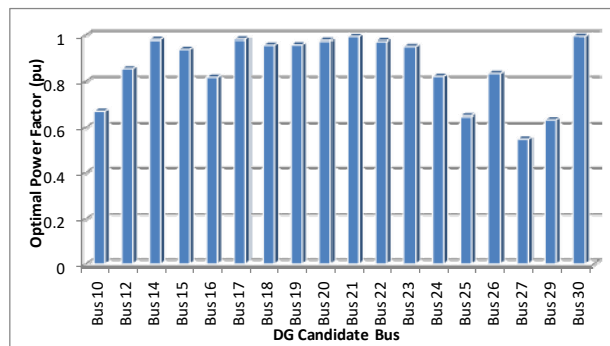
Fig. 3 Optimal Power Factor for DG at Allied Bus
