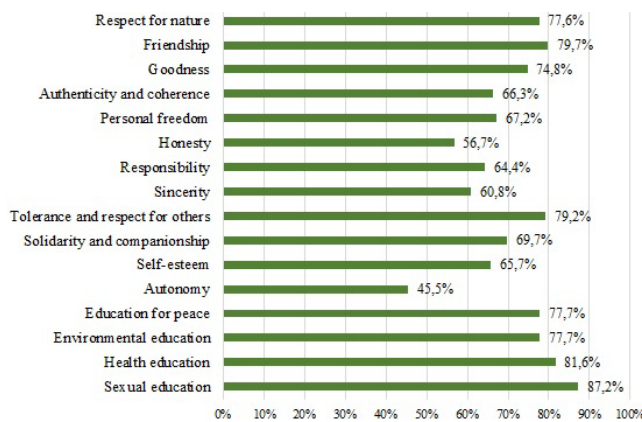
Fig. 3 Percentage of values in students
