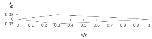
Fig. 20 Diamond airfoil [11]
