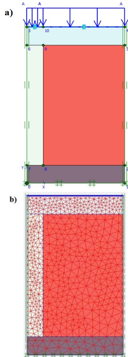
Fig. 2 Axisymmetric numerical model in static analysis, (a) compression loading, (b) mesh sizes in static analysis
