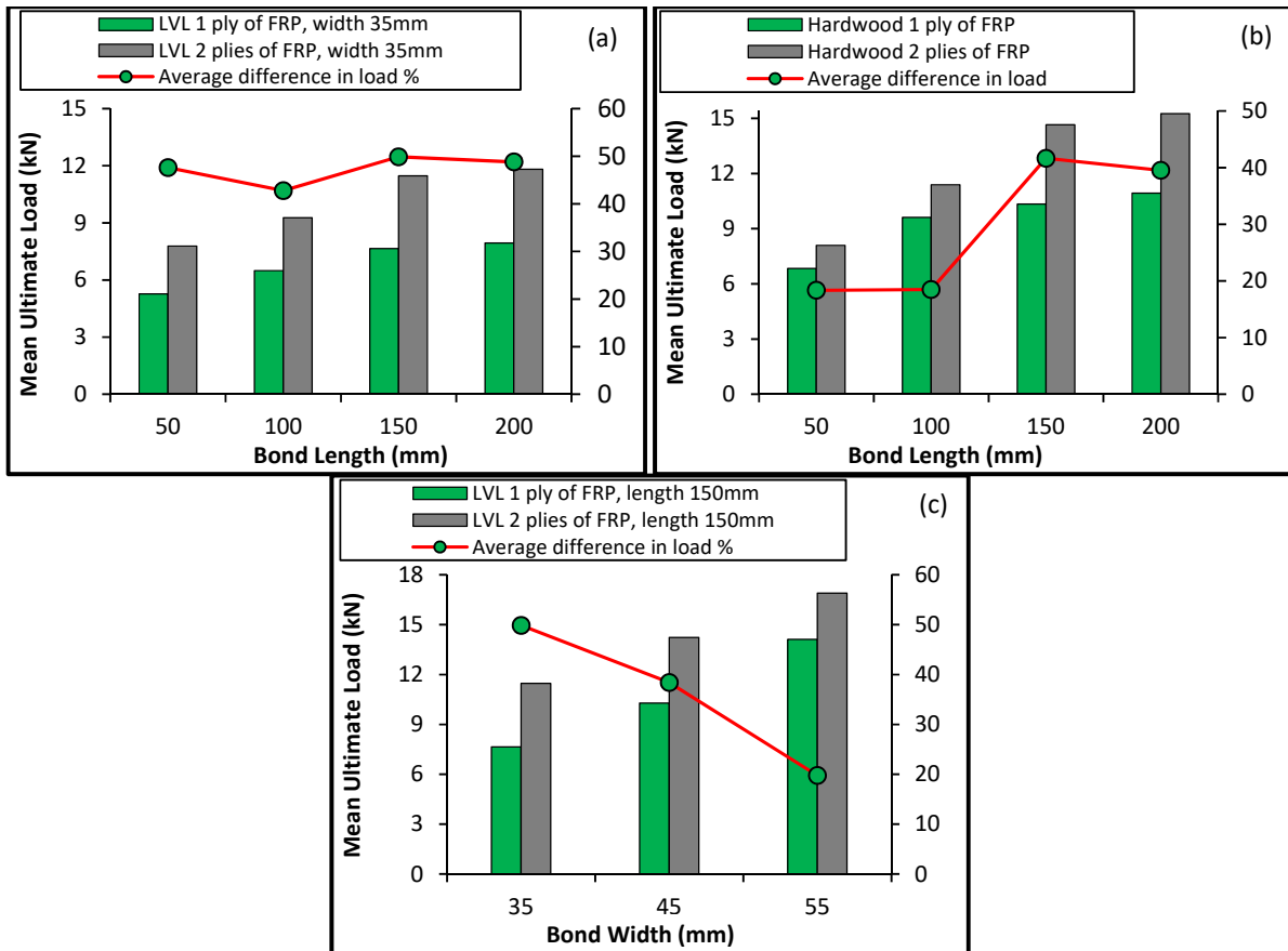
Fig. 5 Relationship between bond strength and bond thickness
