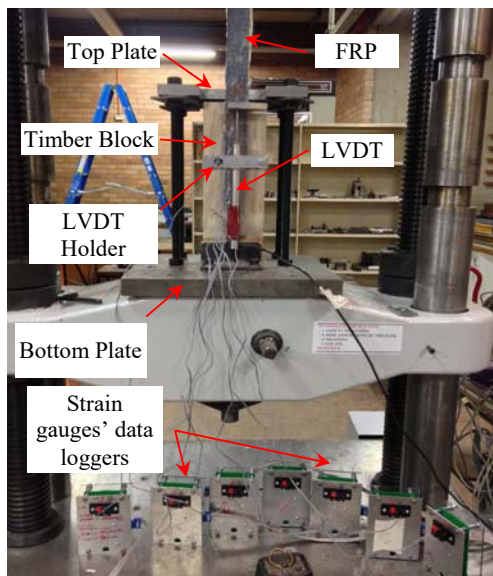
Fig. 1 Modified single shear test setup
