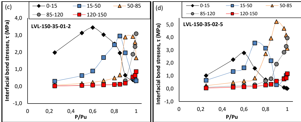
Fig. 4 Relationship between bond stress and bond thickness
