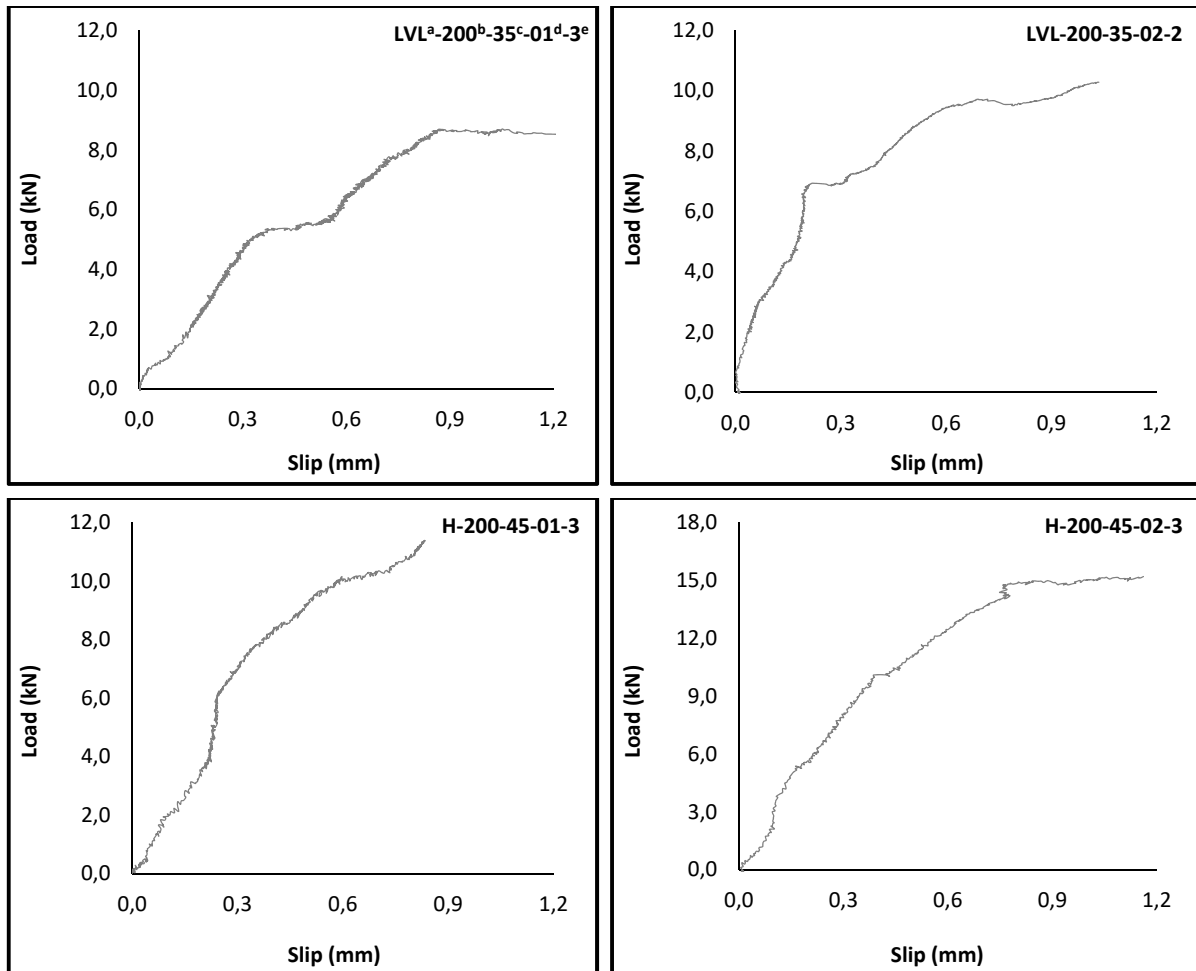
Fig. 2 Load-slip response related to bond thickness series
