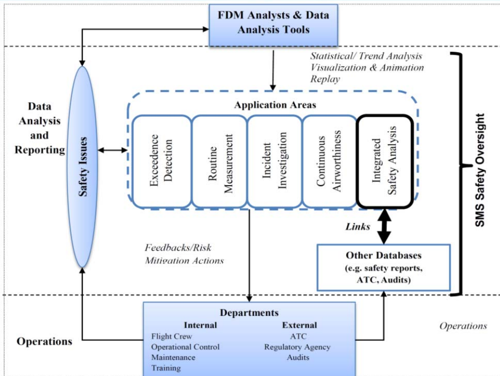
Fig. 1 FDM process [5]
