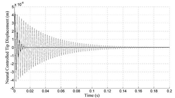
Fig. 8 Vibrations of a cantilever beam with two piezoelectric layers under the neural feedback control
