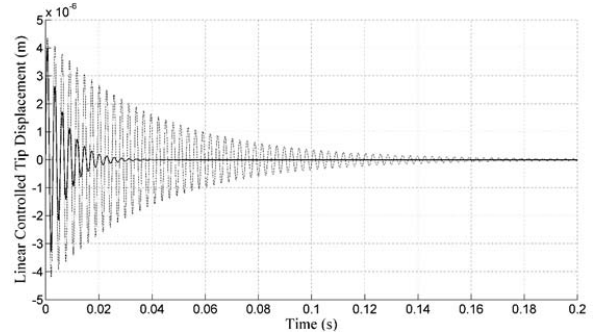
Fig. 7 Vibrations of a cantilever beam with two piezoelectric layers under the linear feedback control
