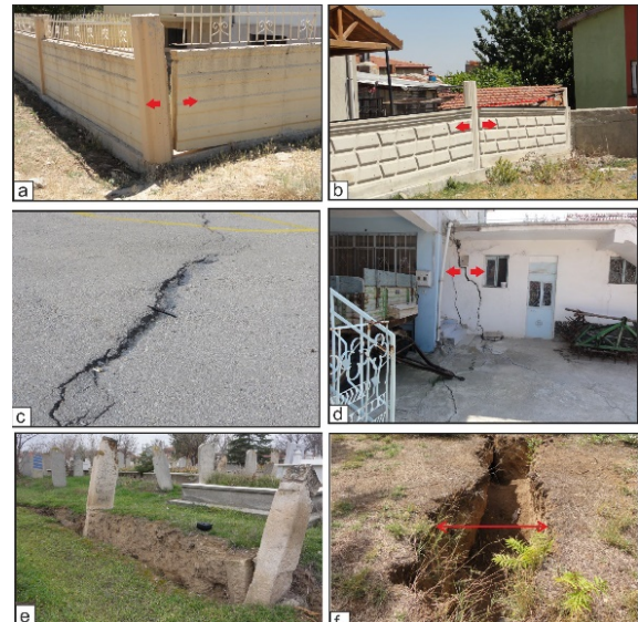
Fig. 3 The Surface deformations observed within the Bolvadin settlement area: (a),(b) The divergence of garden walls of some buildings located on the surface fault near the Park Akcan, (c) Linear deformations on asphalt pavement of the school garden, (d) Extensional cracks in some buildings located on the surface fault (e), (f) Deformations on graves
