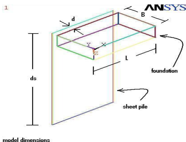
Fig. 3 Model Dimensions
