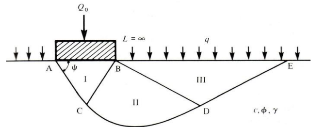
Fig. 2 Failure Wedge (after [2])
