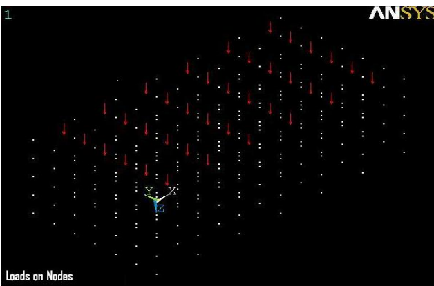
Fig. 5 Applied Loads at the Foundation Nodes
