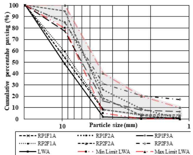
Fig. 5 Gradation curve for LWA and RPA
