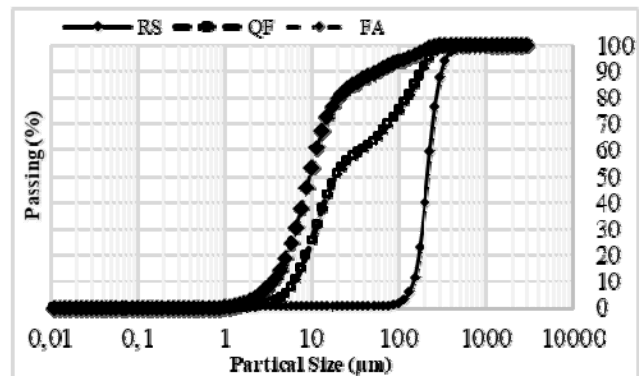
Fig. 2 Particle size distribution of different fillers
