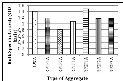
Fig. 7 Bulk specific gravity of various aggregates
