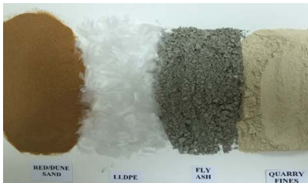
Fig. 1 Plastic and fillers used in manufacturing RPA
