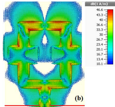
Fig. 3 Simulated (a) radiation pattern characteristics of the antenna at 38 GHz and (b) current distribution
