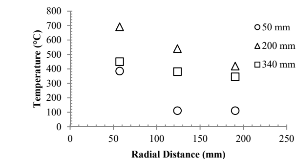
Fig. 4 Temperature distribution in radial direction of the biochar kiln at the height of 50 mm, 200 mm, and 340 mm from the bottom of the kiln with core puncture diameter of 3.18 mm
