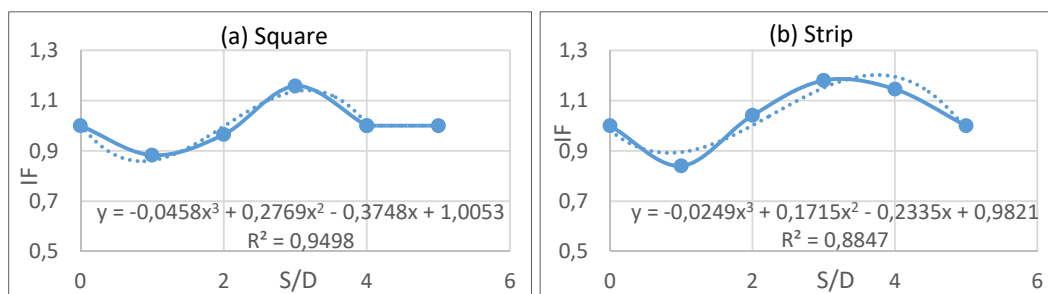
Fig. 4 The diagram of variations of the interference coefficient with distance ratio for (a) square foundation (b) strip foundation
