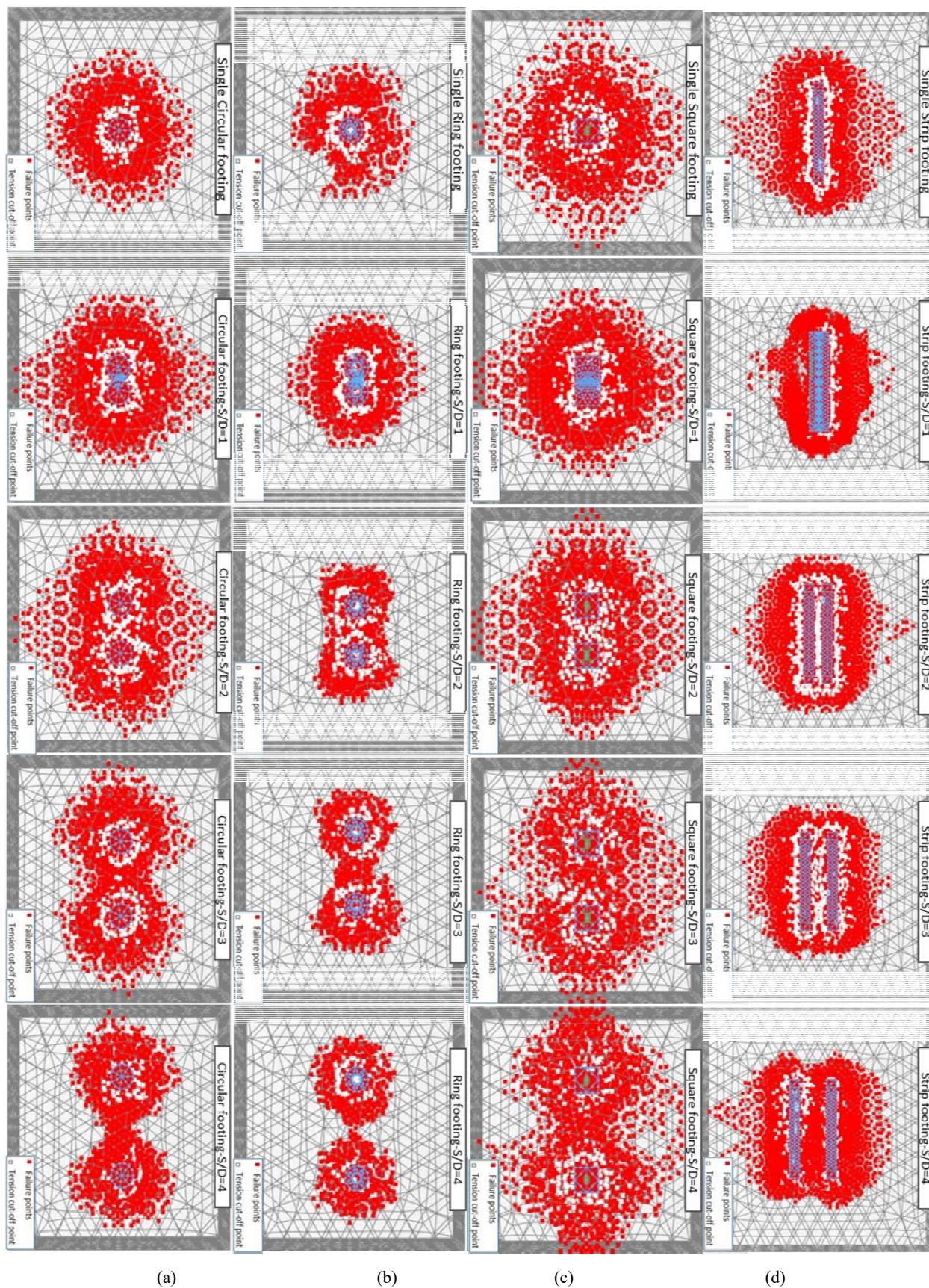
Fig. 5 Plan view of distribution of plastic points based on Mohr Coulomb surrounding the footings as isolated (at top) and S/D ratios of 1 to 4 (a) Circular footing (b) Ring footing (c) Square footing (d) Strip footing
