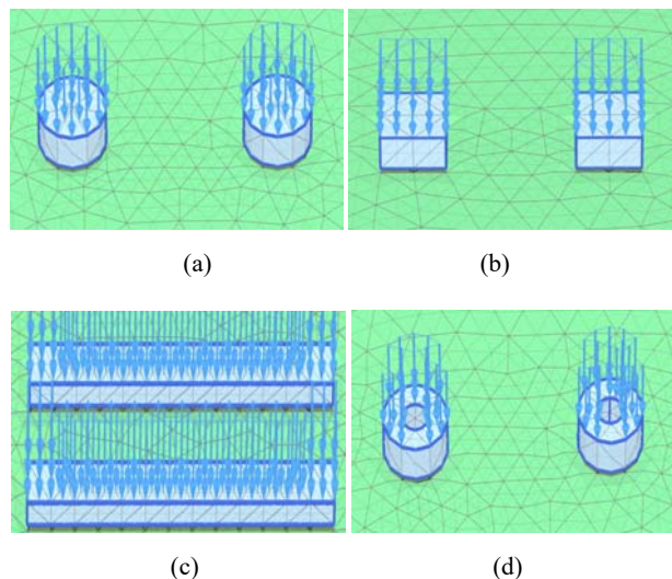
Fig. 1 Geometry, meshing and loading of the (a) Circular foundation model for S/D=3, D=2m. (b) Square foundation model for S/D=3, B=2m. (c) Strip foundation model for S/D=3, B=2m, L=20 m. (d) Ring foundation model for S/D=3, Dout=2 m, Dint=0.8 m
