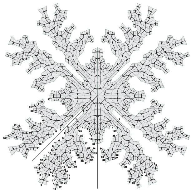
Fig. 4 The hypercube
