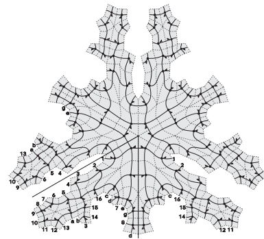
Fig. 3 The hypertetrahedron
