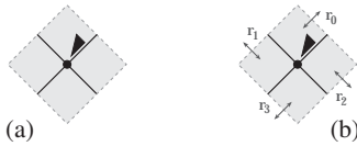
Fig. 1 A rooted \Gamma_4 -slice (a) and sides identification (b)
