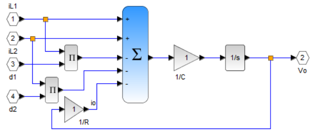
Fig. 8 Block diagram for output voltage
