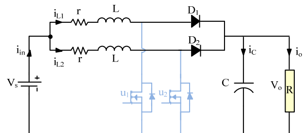
Fig. 5 Equivalent circuit for Mode 4
