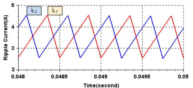
Fig. 19 The steady-state waveforms of inductor current with 180 degree phase shift for D=0.7
