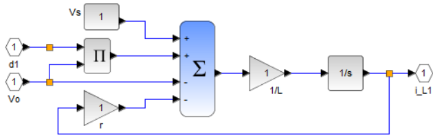
Fig. 6 Block diagram of inductor input current
