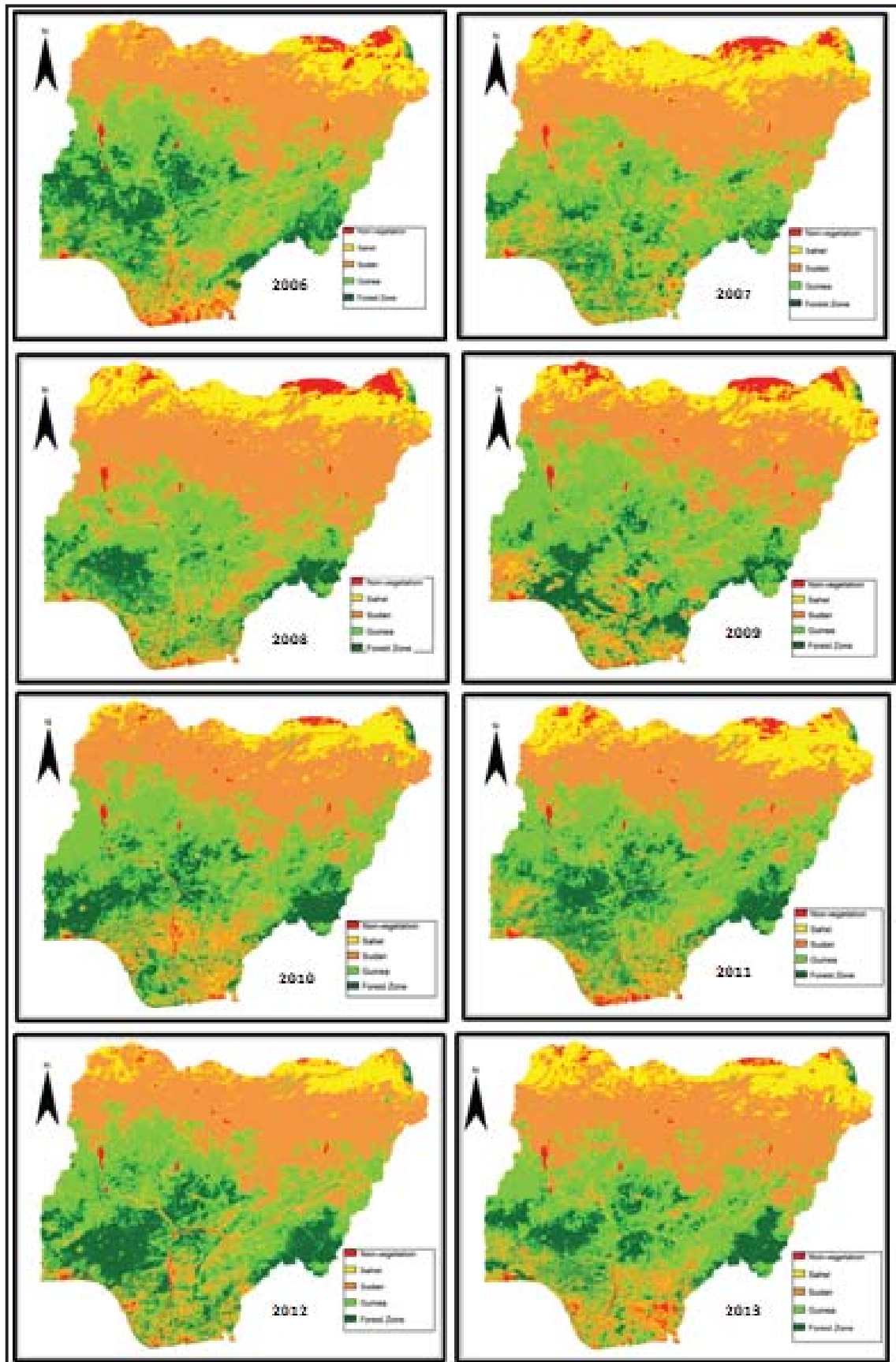
Fig. 3 Vegetation Zones (2006-2013)
