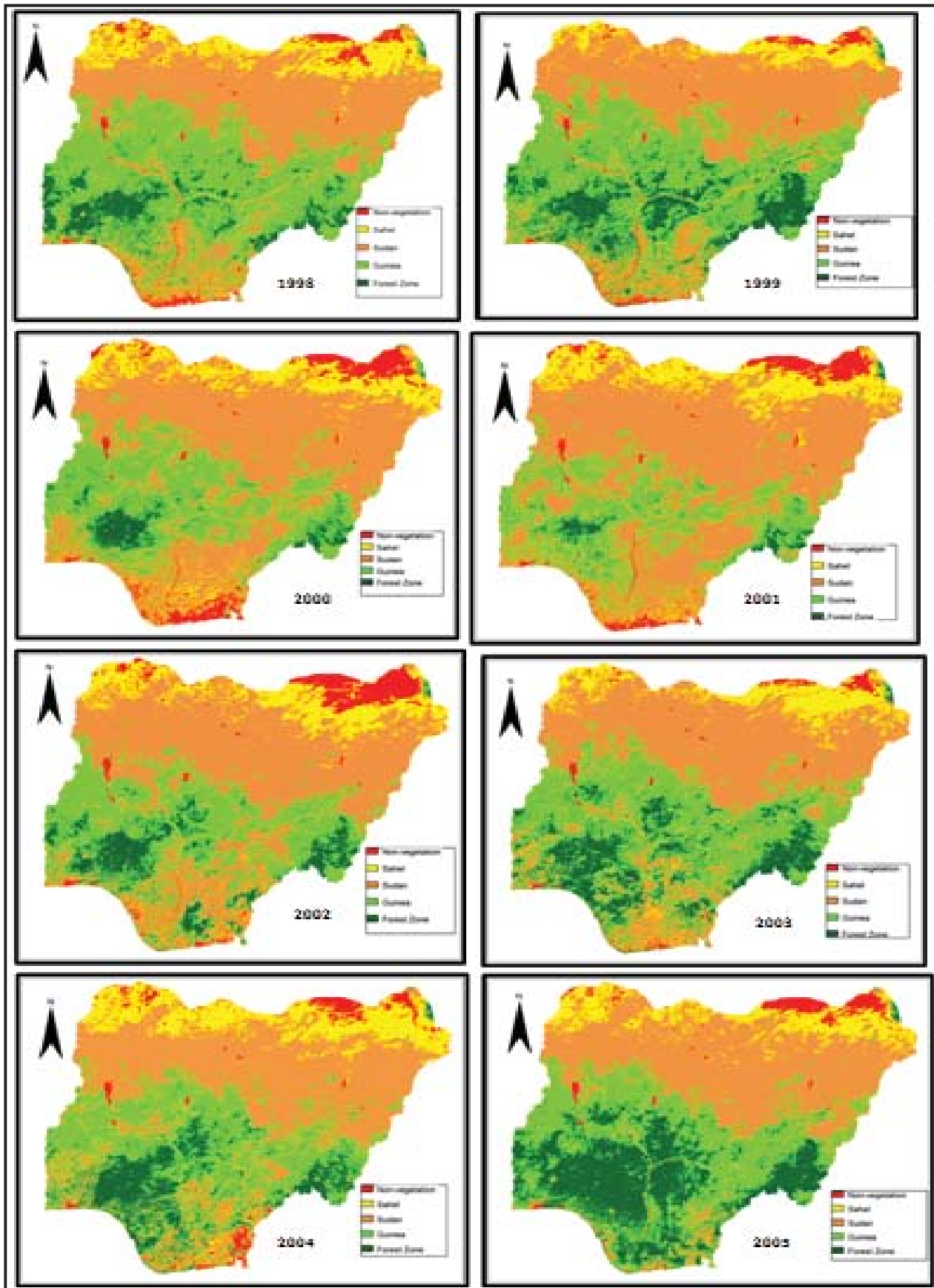
Fig. 2 Vegetation Zones (1998-2005)
