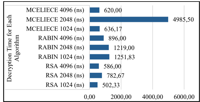
Fig. 9 Decryption time for each algorithm
