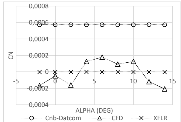
Fig. 7 Comparison between coefficient of yawing moment from XFLR and DATCOM
