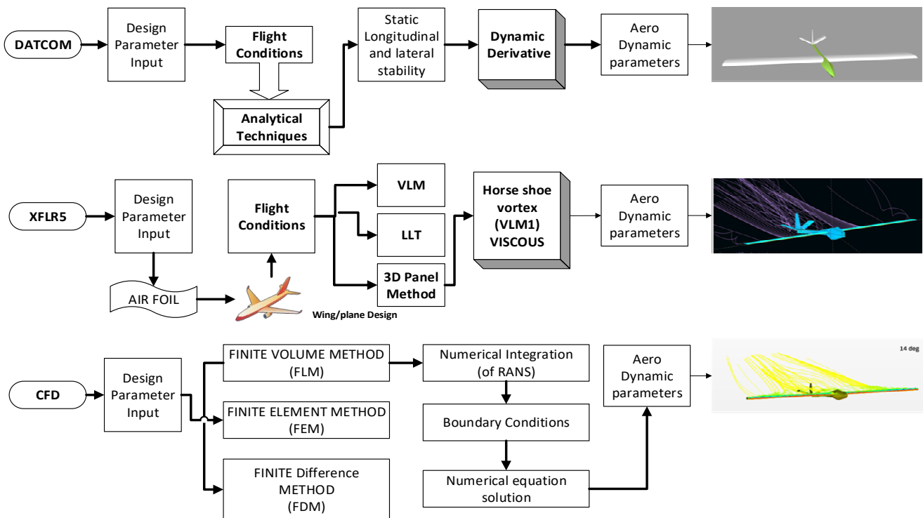
Fig. 1 Schematic layout of the techniques used for processing aerodynamic variables i.e. top is DATCOM, middle is XFLR and last is the CFD process.
